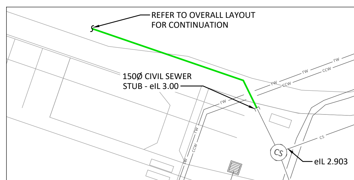
SANITARY DRAINAGE INSET SCALE 1:200
